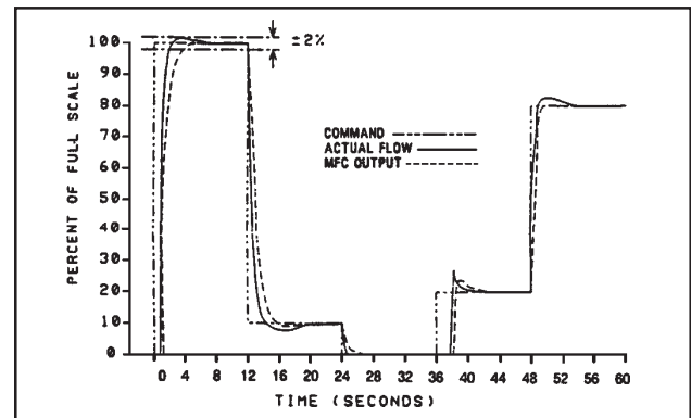
Model 5850E Performance Curve (1 slpm N 2 @ 25 psig)
